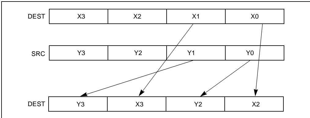
Figure 3-22. UNPCKLPS Instruction Low Unpack and Interleave Operation
