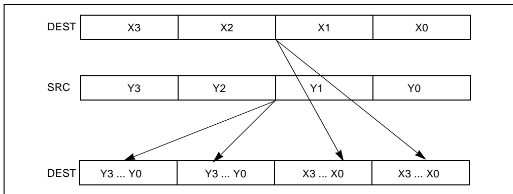
Figure 3-18. SHUFPS Shuffle Operation
