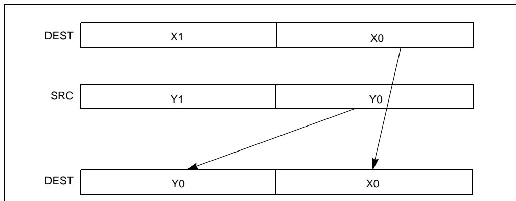
Figure 3-21. UNPCKLPD Instruction Low Unpack and Interleave Operation
