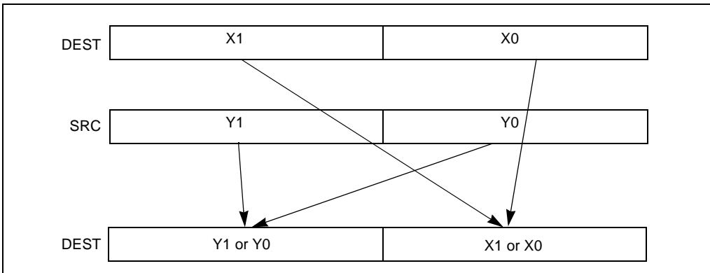
Figure 3-17. SHUFPD Shuffle Operation
