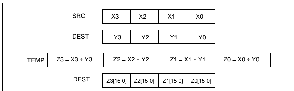
Figure 3-9. PMULLU Instruction Operation Using 64-bit Operands
