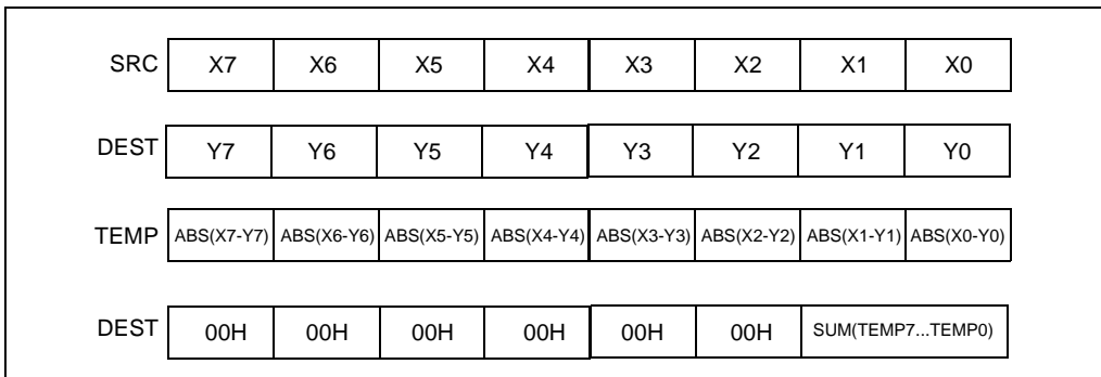
Figure 3-10. PSADBW Instruction Operation Using 64-bit Operands
