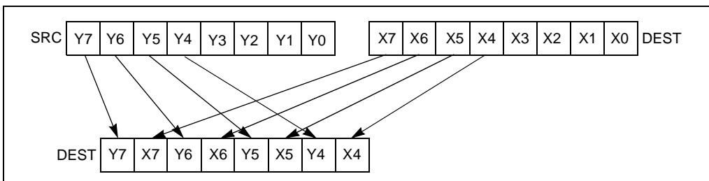
Figure 3-15. PUNPCKHBW Instruction Operation Using 64-bit Operands
